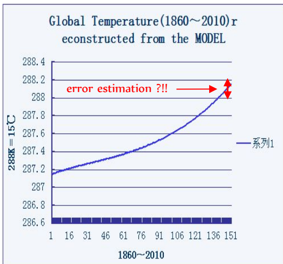
The verification curve in actual past data of temperature with CO2 concentration.
